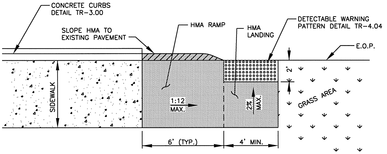
ATTACHED SIDEWALK
