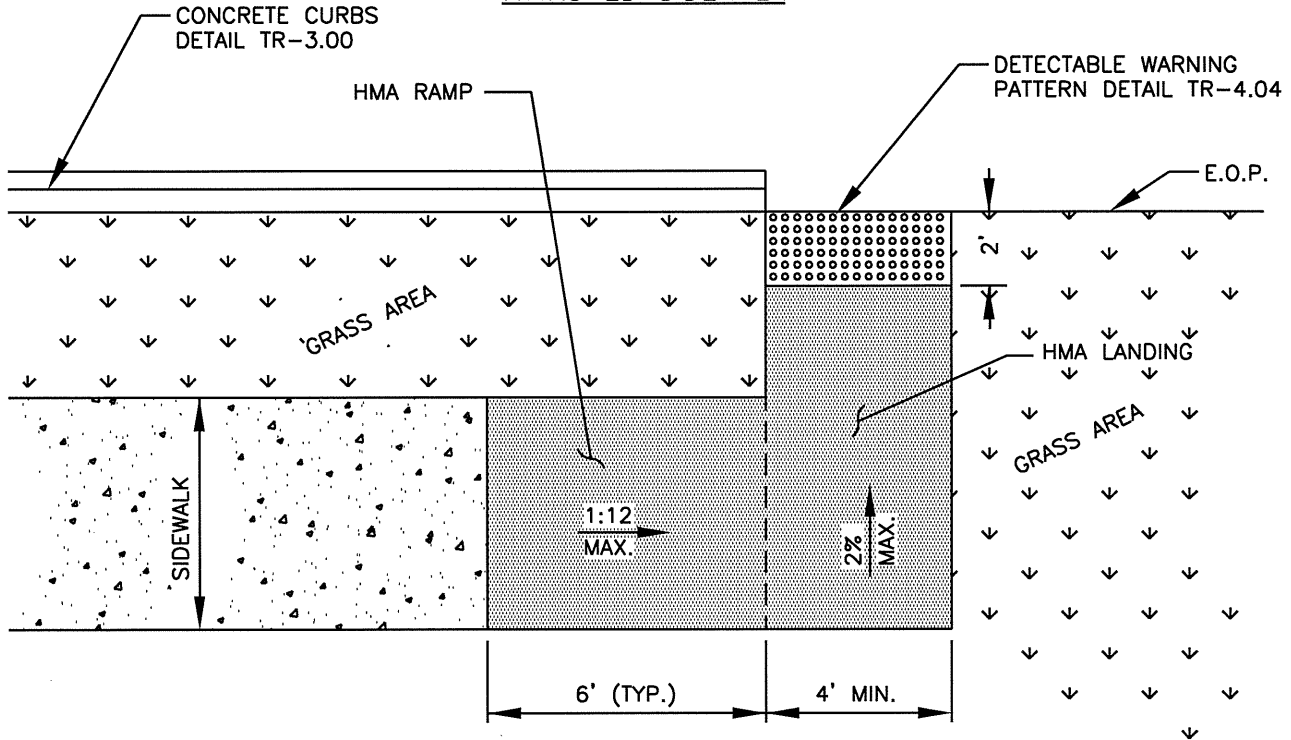
DETACHED SIDEWALK
