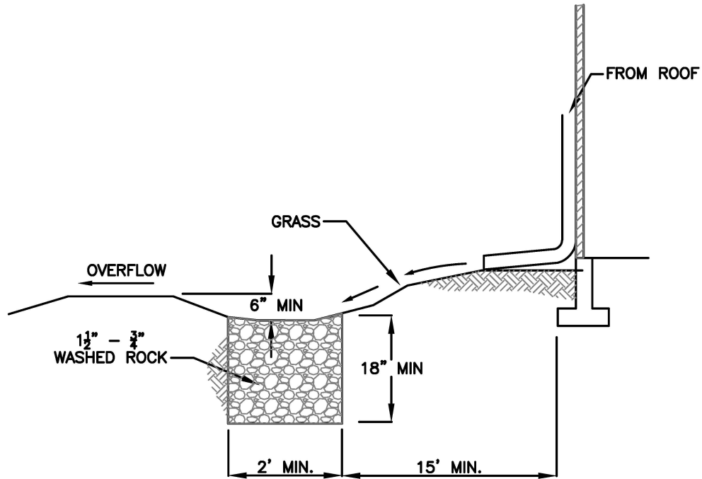
CROSS SECTION
