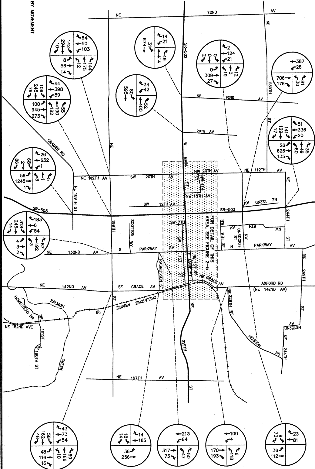
Figure 2-4 Existing PM Peak Hour Traffic Volumes CITY OF BATTLE GROUND TRANSPORTATION SYSTEM PLAN
