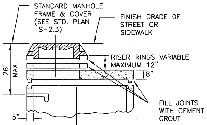
FLAT SLAB ALTERNATE
