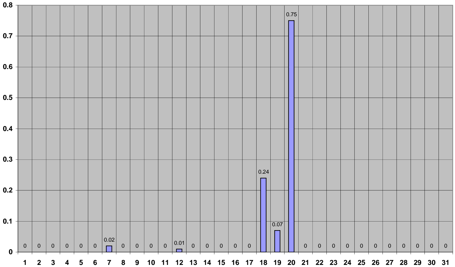
Battle Ground Precipitation August 2007
